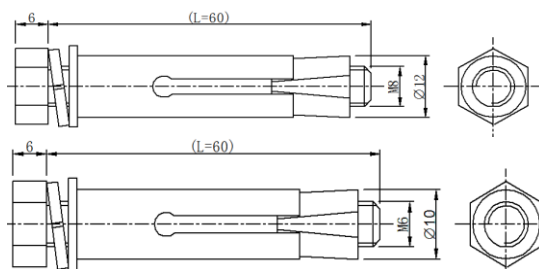
M6/M8 膨胀螺丝尺寸参考图
